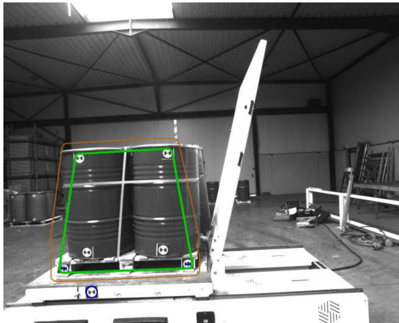
Permanent Deformation
