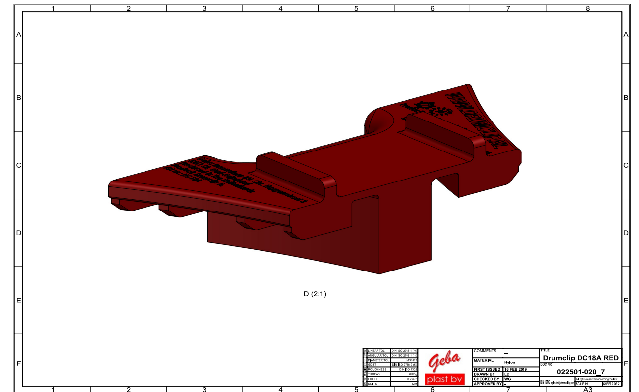
Figure 7b: Isometric view DRUMCLIP DC18A RED
