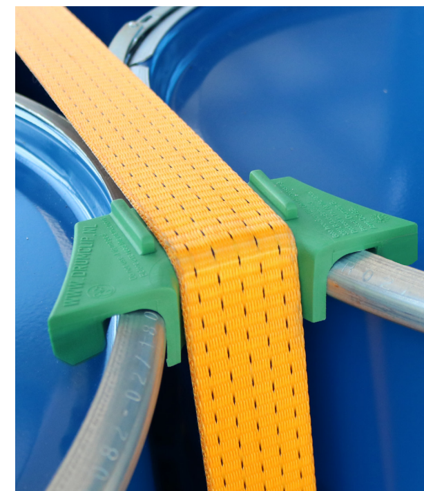
Figure 18: DRUMCLIP DC19B GREEN secured with universal lashing strap.
