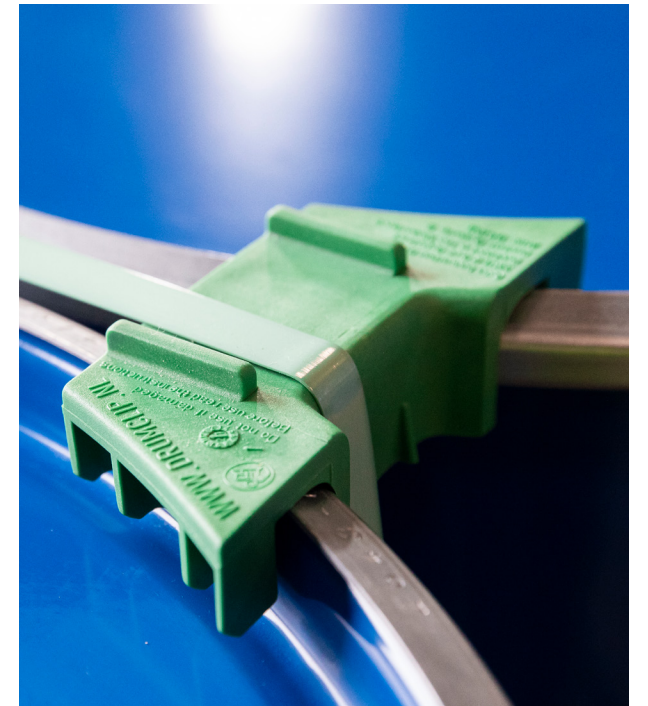
Figure 17: DRUMCLIP DC19B GREEN secured with Signode Tenax T2220 Polyester strap
